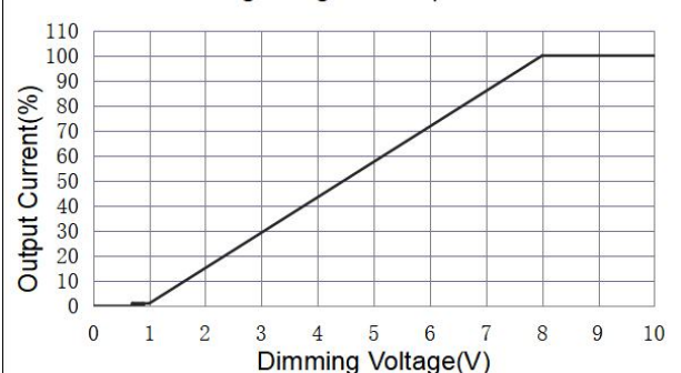
Dimming Voltage Vs. Output Current
