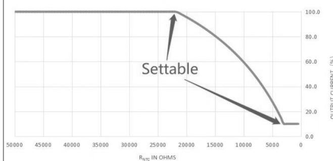
LED OTP Curve
