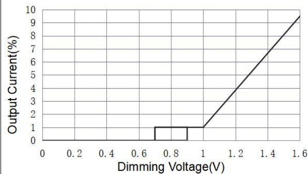
Dimming Voltage Vs. Output Current
