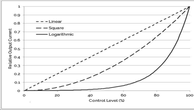
Figure 1: Intensity Dimming Profile Characteristics
