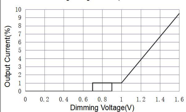
Dimming Voltage Vs. Output Current
