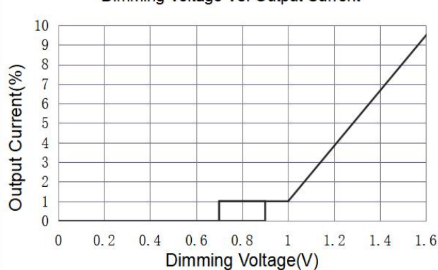
Dimming Voltage Vs. Output Current
