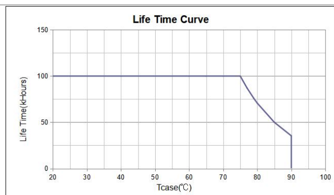
AFP-B1-025 and AFP-B1-040 life time curve
